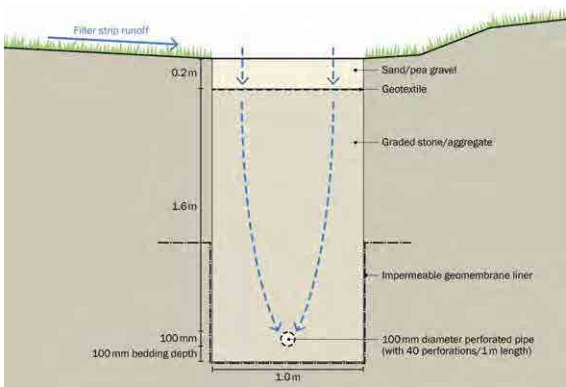
Figure C.14 Lorry park filter drain
