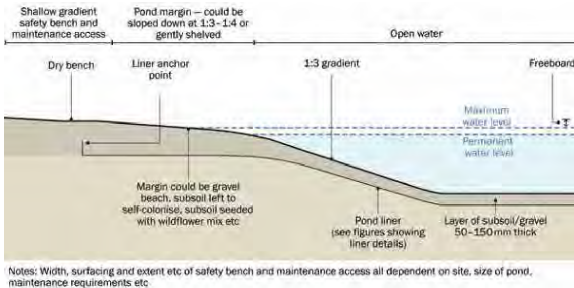
Figure 23.6 Typical non-planted pond edge details
