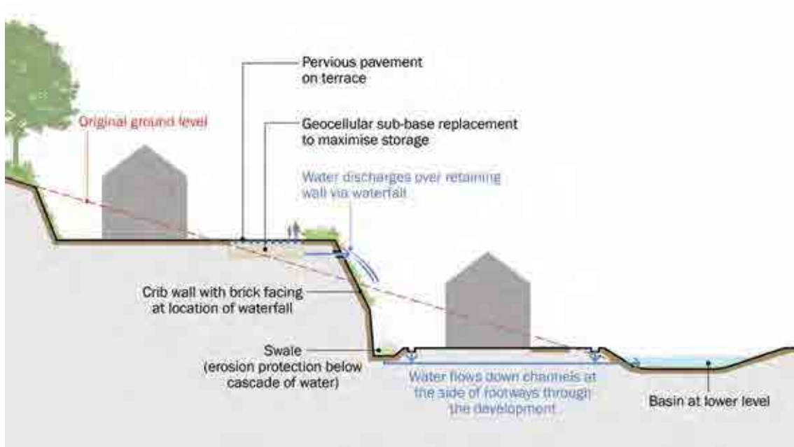
Figure 8.6 Cross-section showing example SuDS on a sloping site
