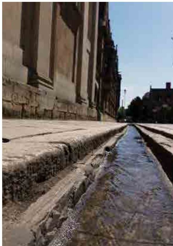
Figure 10.18 Roadside rills, Cambridge (courtesy Cambridgeshire County Council)
