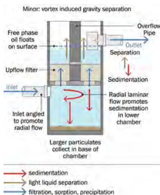
Figure 14.12 Multi-process system
