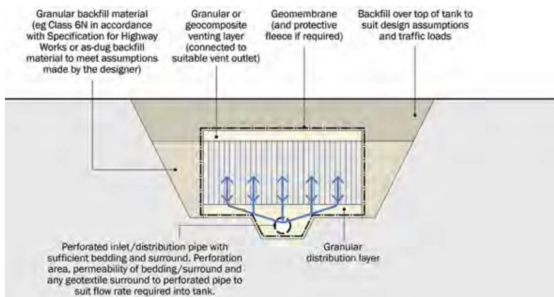
Figure 21.7 Schematics of 2D systems in attenuation storage mode (upflow filling)
