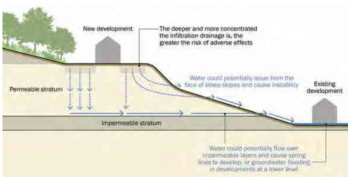
Figure 8.9 Impact of geology on water flows from infiltration drainage on sloping sites
