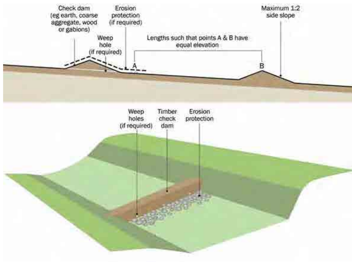
Figure 17.13 Typical check dam details
