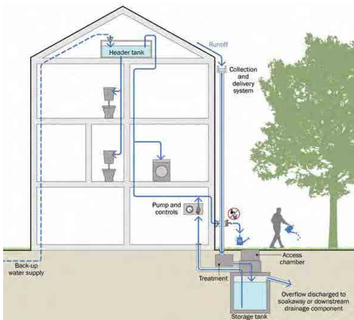
Figure 11.4 A conceptual pumped rainwater harvesting system
