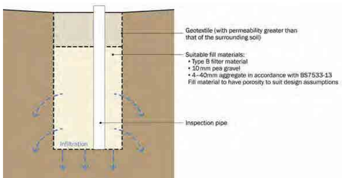
Figure 13.3 Infiltration trench
