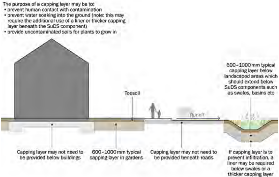
Figure 8.1 Contaminated land and SuDS: typical capping layers
