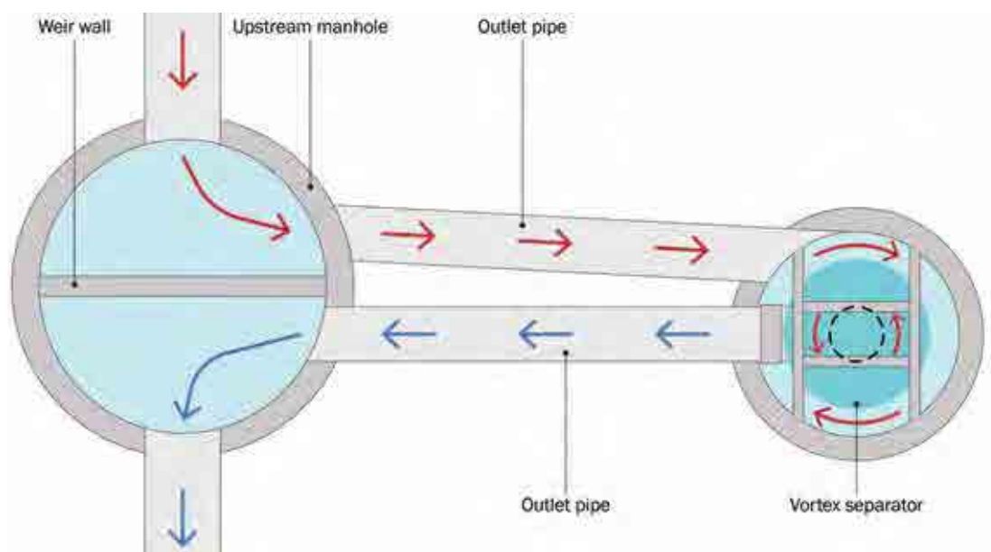
Figure 14.5 Hydrodynamic separator with a separate external bypass (courtesy Hydro International)
