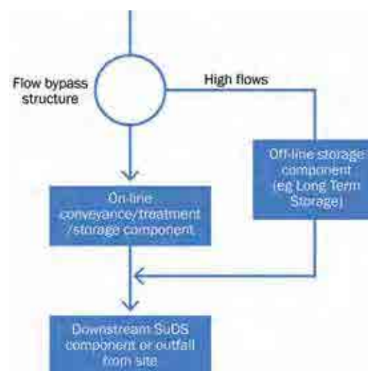
Figure 28.9 Requirements for flow bypass structures
