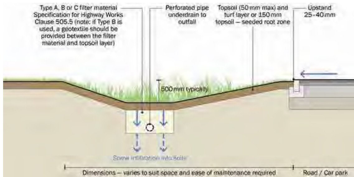
Figure 9.15 Swale detail
