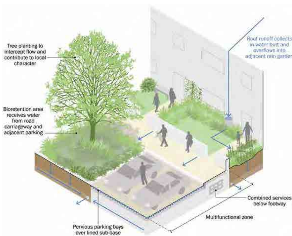
Figure 10.16 Multi-functional streetscape
