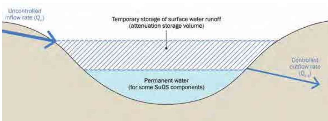
Figure 3.2 Controlling runoff rates using attenuation storage
