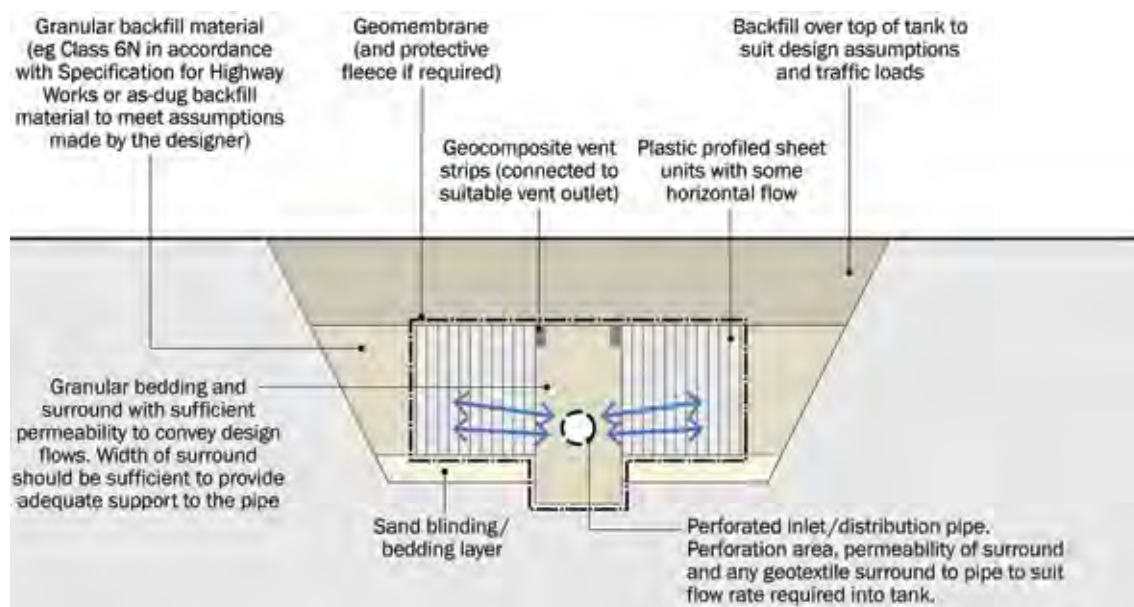
Figure 21.6 Schematic of 2D system in attenuation storage mode (central inlet pipe)
