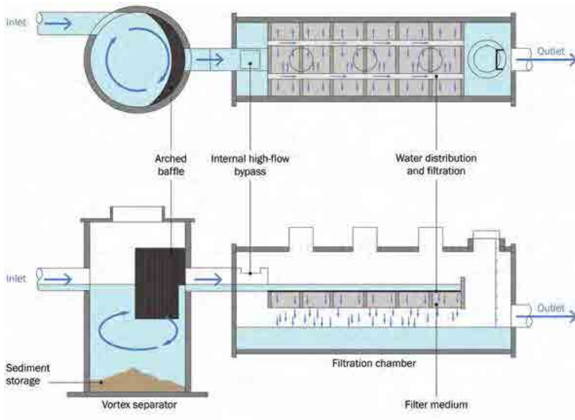
Figure 14.8 Schematic of a vortex-enhanced sedimentation and media filtration system
